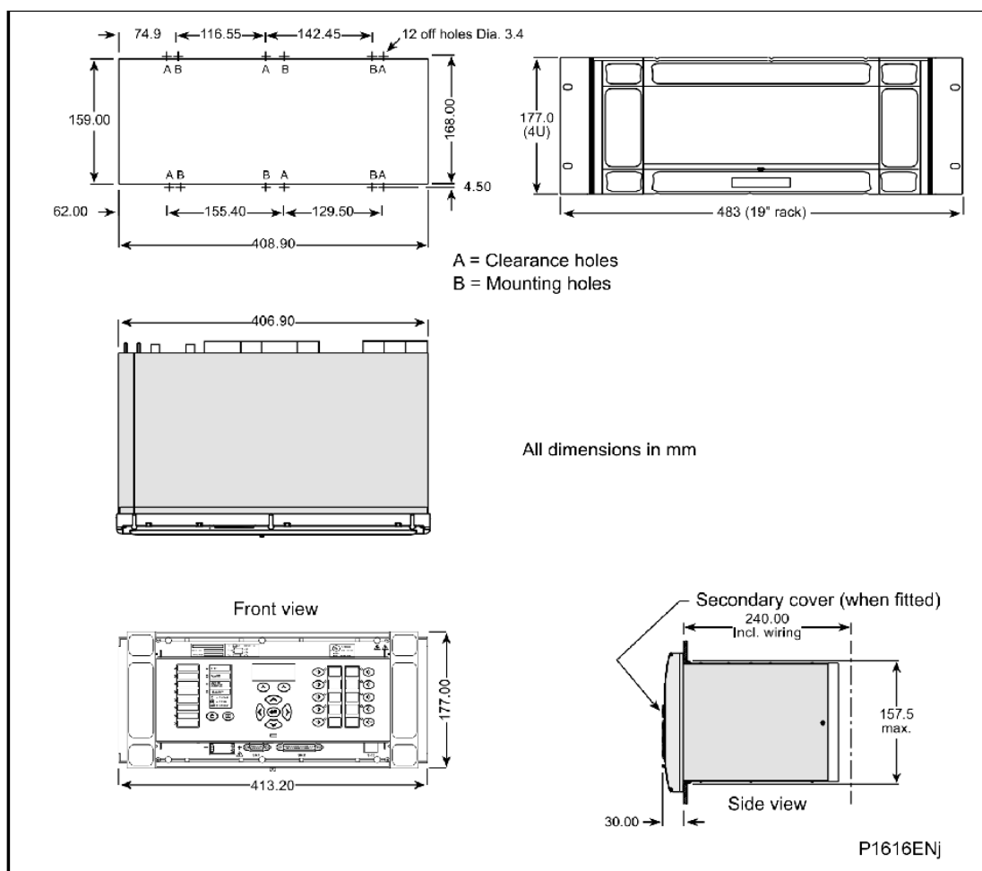
Figure 5 P645 case dimensions (80TE case)
