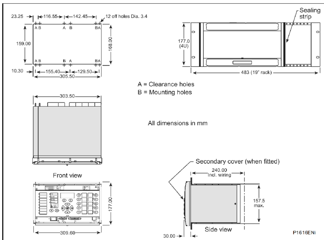
Figure 4 P643 case dimensions (60TE case)
